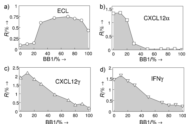
Figure 3. Continuous evolution profiles (CEP) obtained from the CoCRRs array for proteins a) ECL (200 nM), b) CXCL12 \alpha (100 nM), c) CXCL12 \gamma (100 nM) and d) IFN \gamma (25 nM). The recognition patterns were generated by plotting the reflectivity ( R ) at the end of injection versus the \frac{[BB1]}{([BB1] + [BB2])} ratio.
