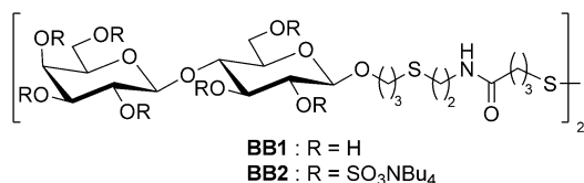
Figure 2. Formulas of the two disulfide building blocks BB1 and BB2 used to construct the combinatorial cross-reactive receptors array.
